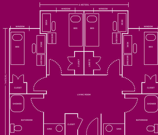
Shocker Hall Floor Plan
